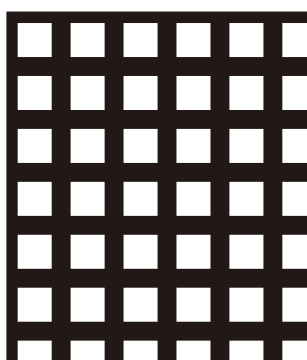
105 4.5□×7.0P 開孔率 41.3%
