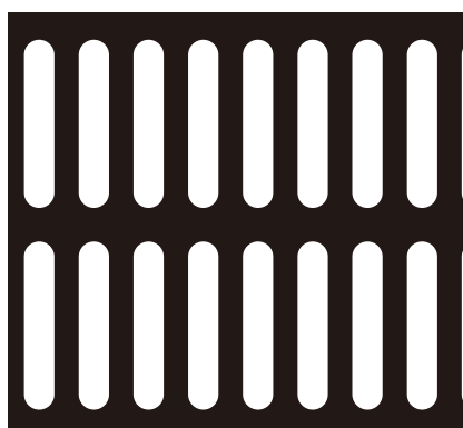
96 (3.6 × 20.0) × (6.5 × 24.5)P 開孔率 44.7%
