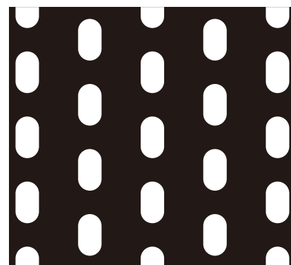
91 (4.5 × 8.0) × (24.0 × 12.0)P 開孔率 24.3%
