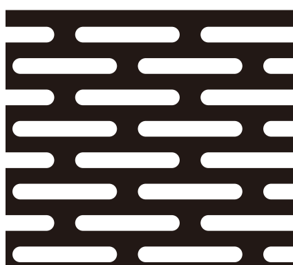
80 (3.0 × 20.0) × (12.0 × 24.5)P 開孔率 40.4%
