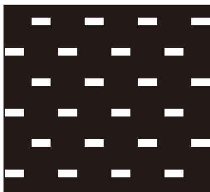
78 [2.0 × 5.0] × [16.0 × 14.0]P 開孔率 8.9%
