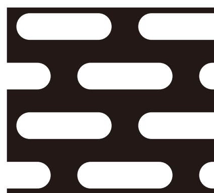
82 (7.0 × 25.0) × (26.0 × 32.0)P 開孔率 41.7%
