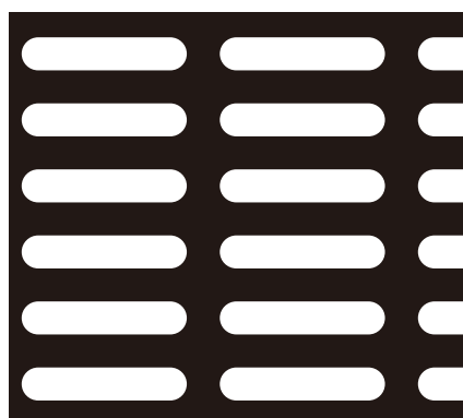
86 (4.0 × 20.0) × (8.0 × 24.0)P 開孔率 41.2%
