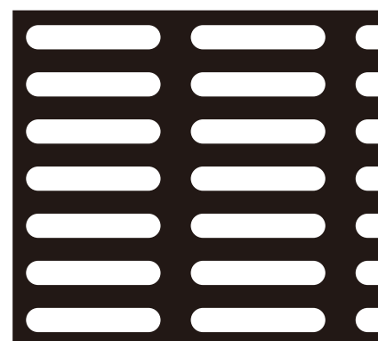
85 (3.6 × 20.0) × (7.0 × 24.5)P 開孔率 41.5%
