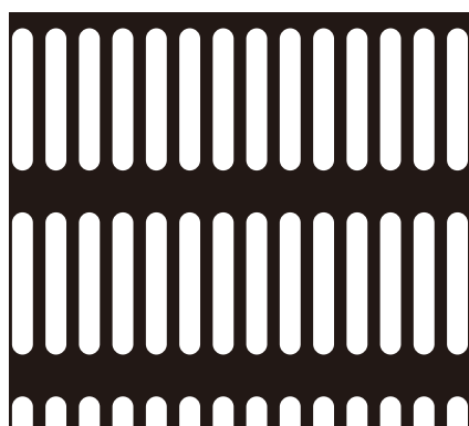
95 (2.5 × 17.0) × (4.0 × 22.0)P 開孔率 47.7%
