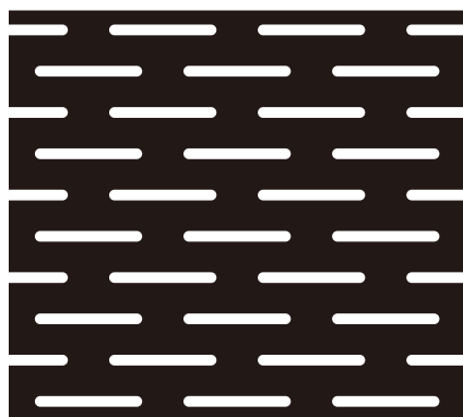
77 (1.3 × 13.0) × (10.0 × 18.0)P 開孔率 18.5%
