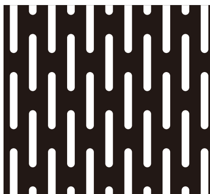
90 (2.0 × 15.0) × (10.0 × 20.0)P 開孔率 29.6%
