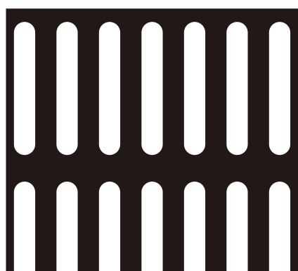
98 (4.0 × 25.0) × (8.0 × 30.0)P 開孔率 41.3%
