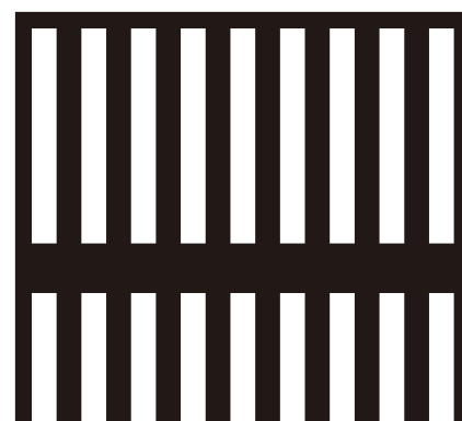
97 [3.0 × 26.0] × [6.0 × 32.0]P 開孔率 40.3%
