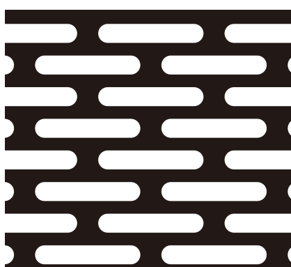
81 (3.6 × 20.0) × (13.0 × 24.5)P 開孔率 44.7%
