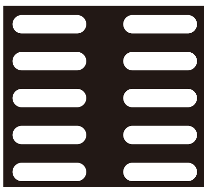
87 (5.0 × 20.0) × (10.0 × 30.0)P 開孔率 33.0%
