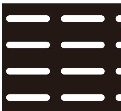
84 (3.0 × 20.0) × (12.0 × 24.5)P 開孔率 20.2%
