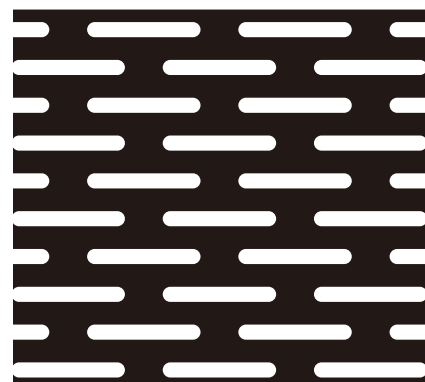
79 (2.0 × 15.0) × (10.0 × 20.0)P 開孔率 29.6%
